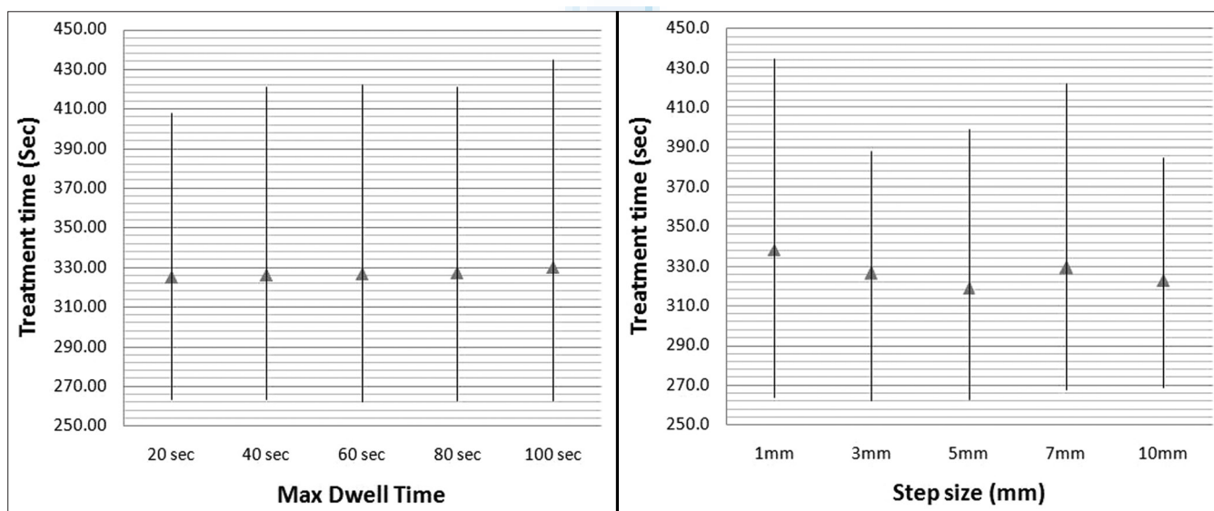
Figure 3: Variation of treatment time with step size and dwell time
